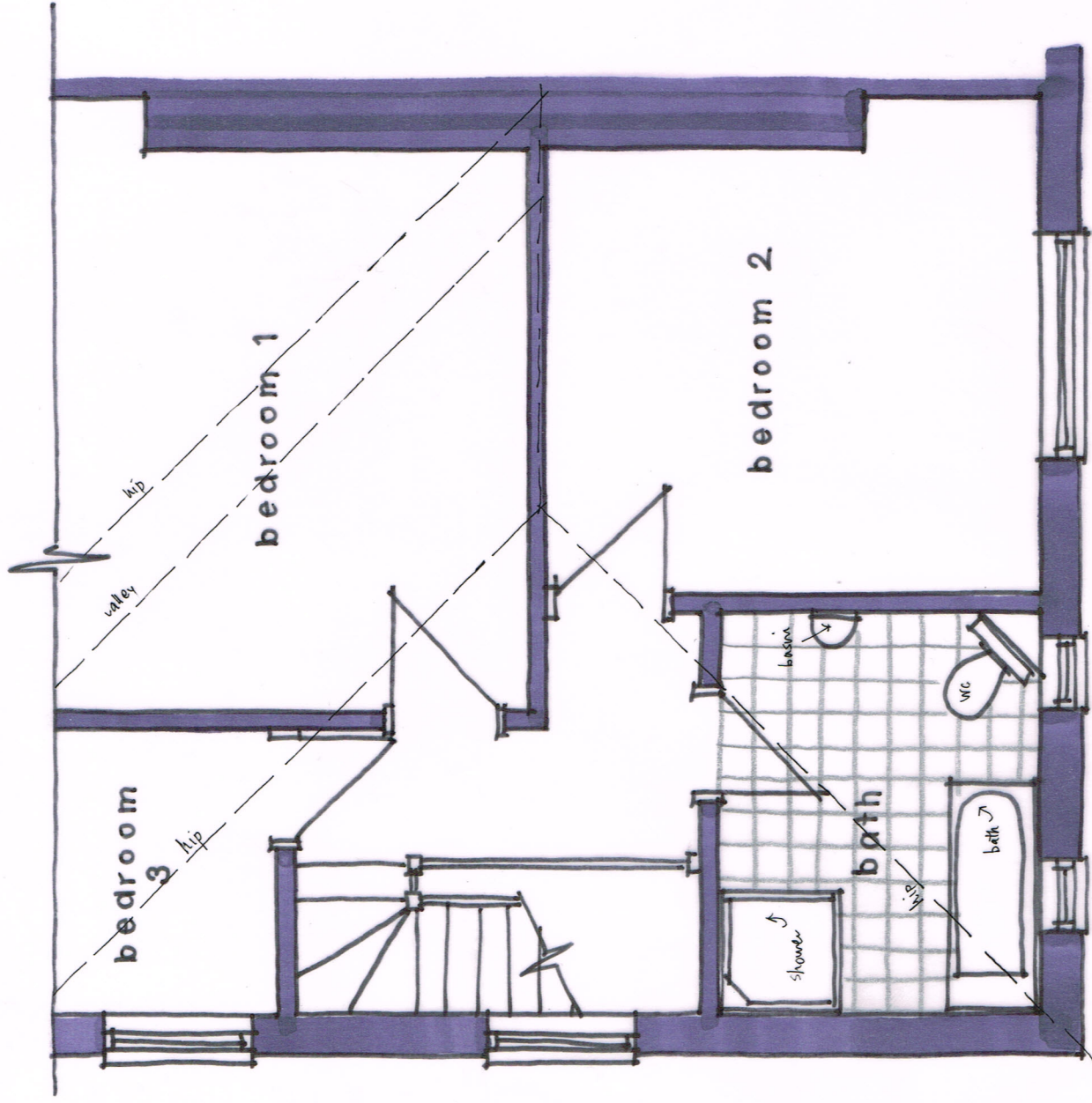
1st FLOOR PLAN 1:50 @ A3 (EXISTING)
