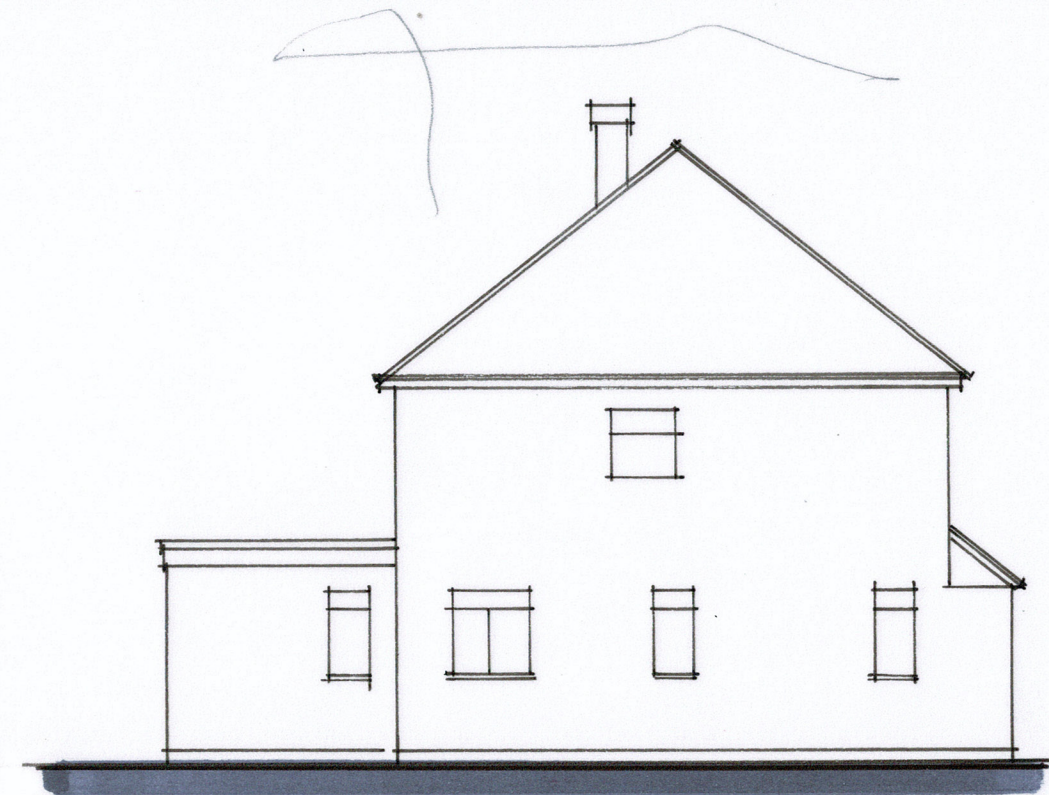
SIDE (e) ELEVATION 1:100 @ A3
