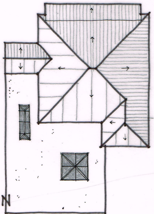
ROOF PLAN 1:200
