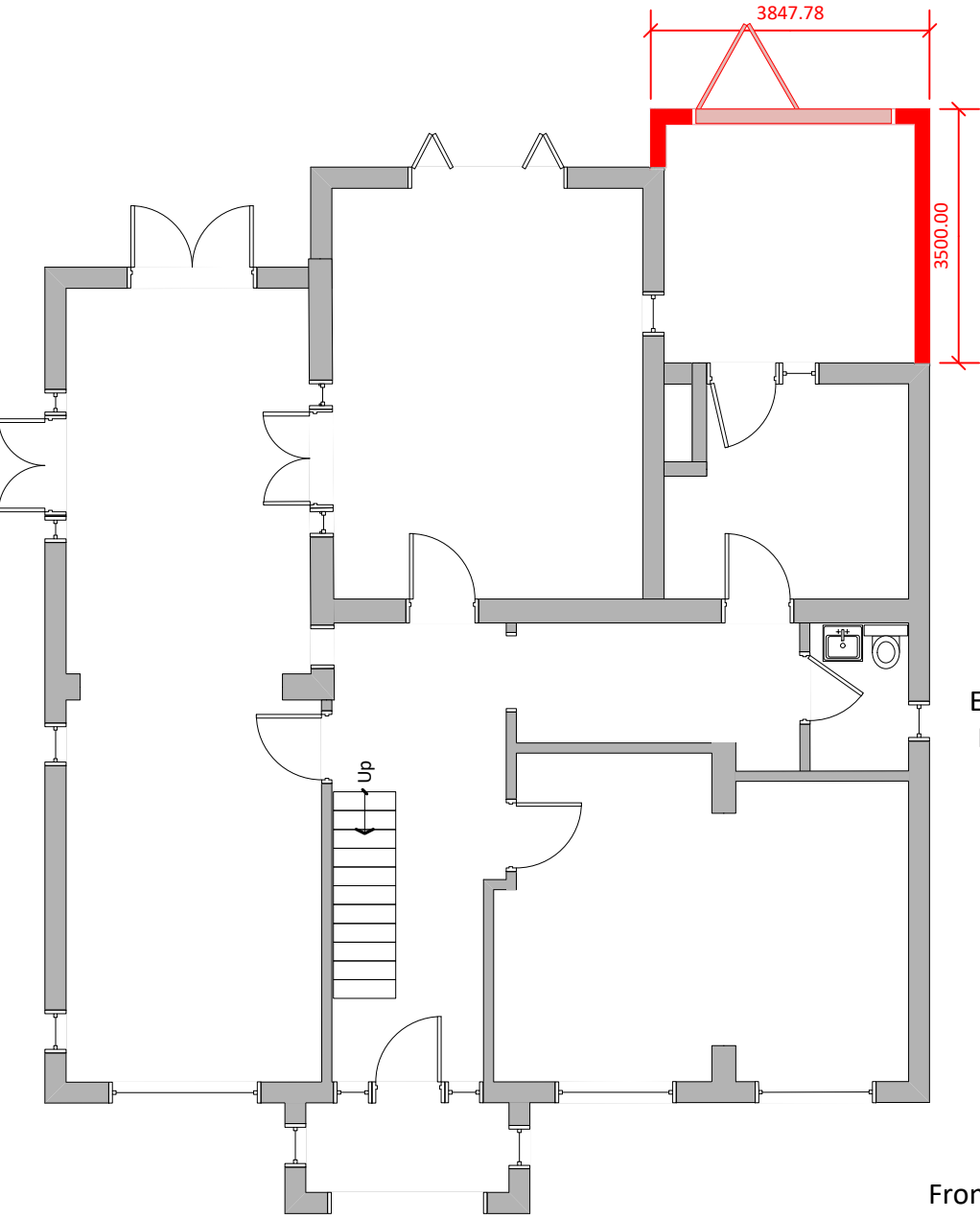
Ground Floor
