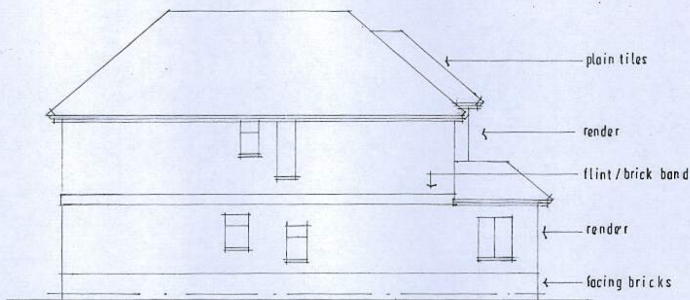
NORTH 1/100
