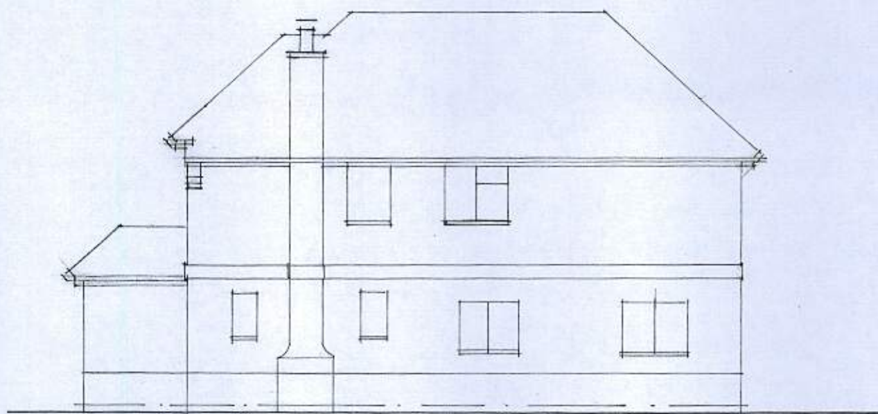
SOUTH 1/100
