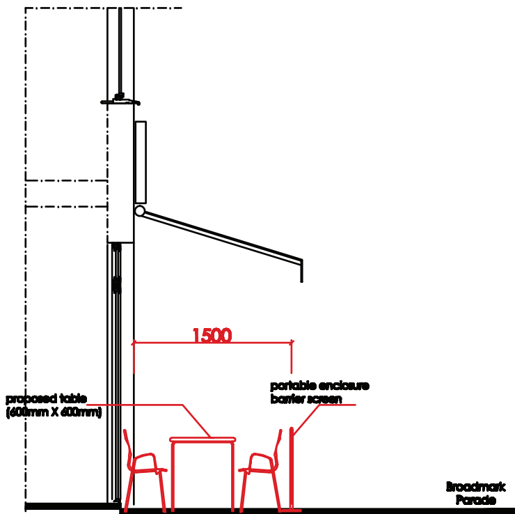
PROPOSED SIDE ELEVATION 1:50
