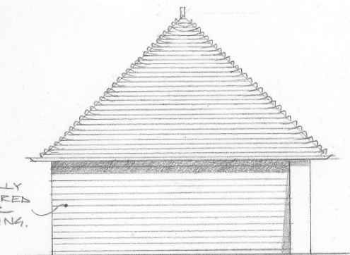
SIDE ELEVATION PLOT 1 (NORTH)
