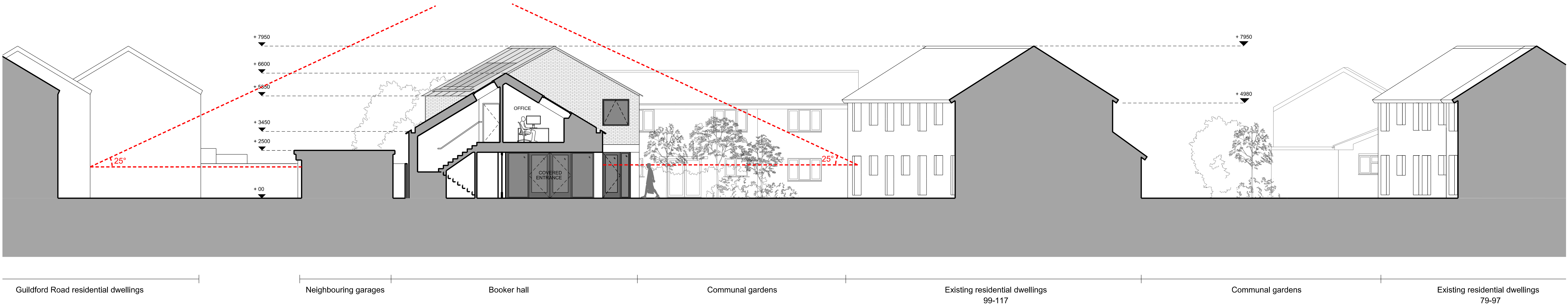
SECTION AA
