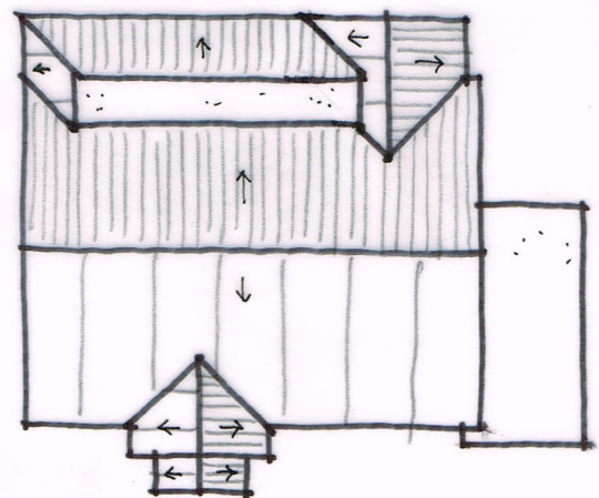
ROOF PLAN 1:200
