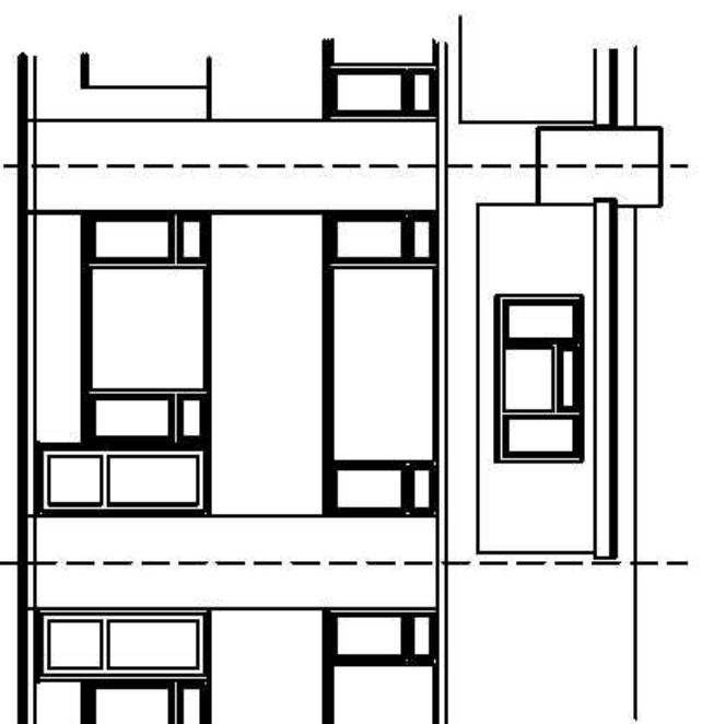
Existing rear elevation west
