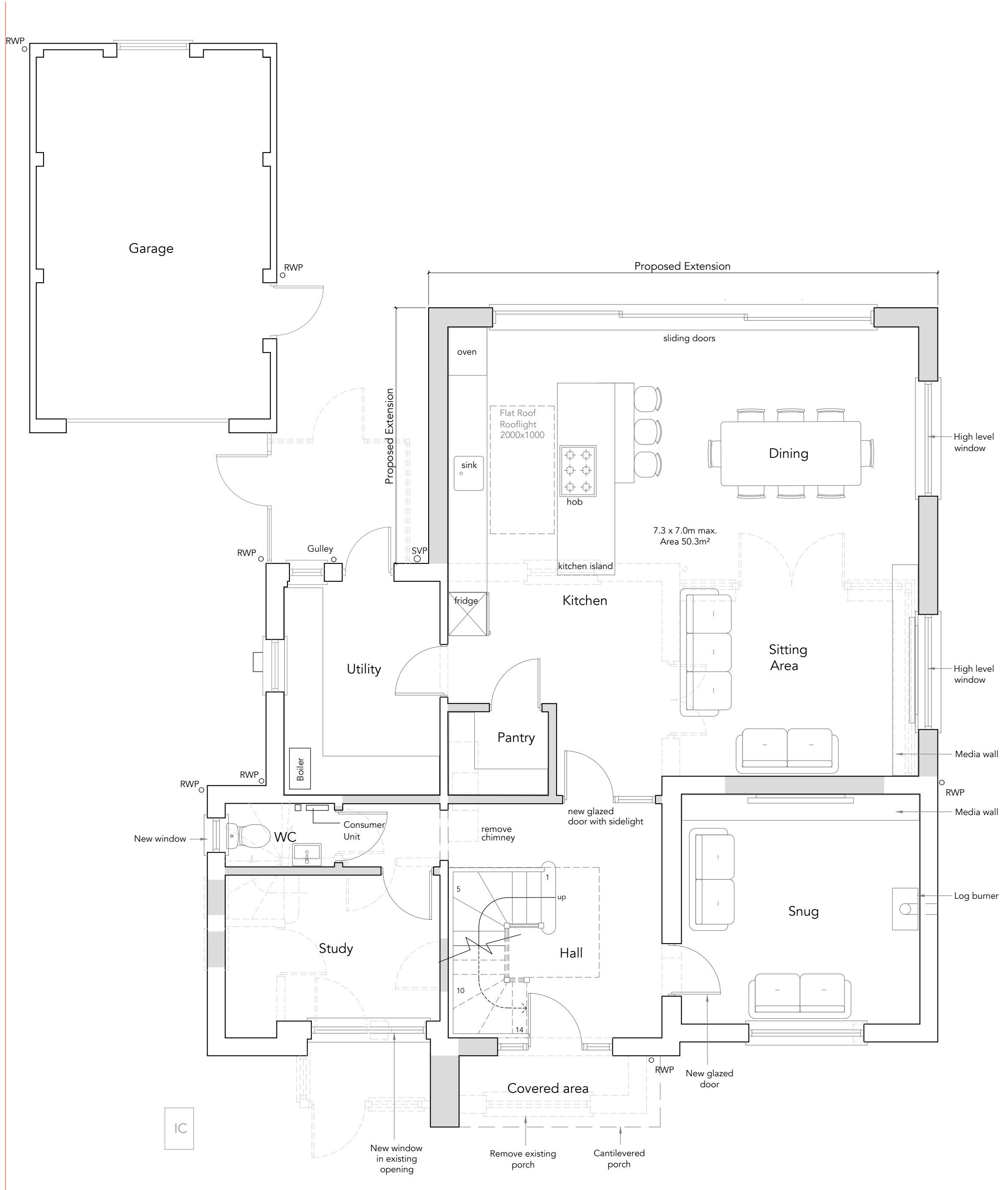
Ground Floor Plan Proposed 1:50
