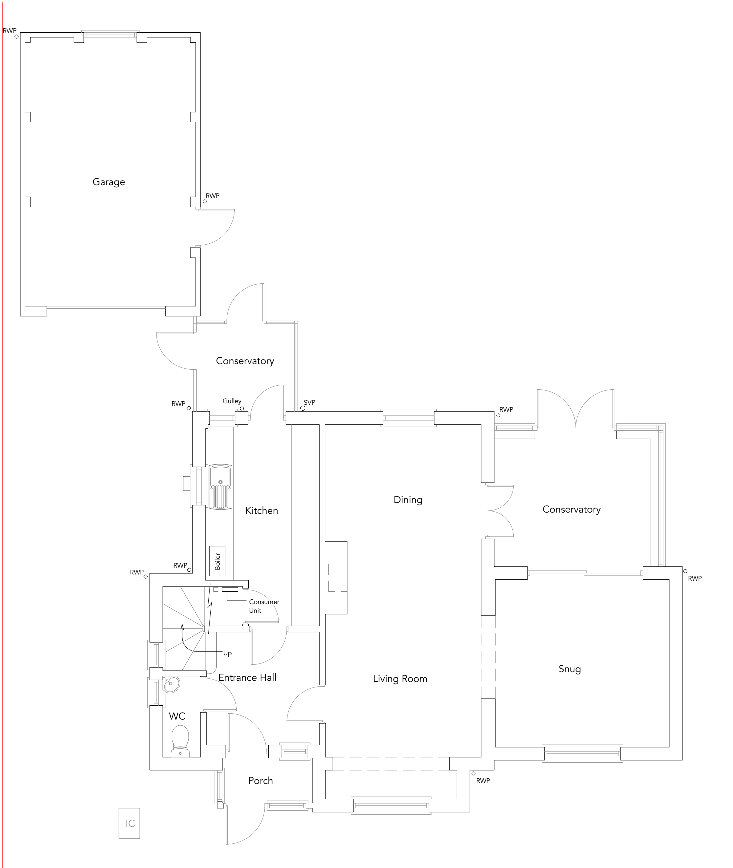
Ground Floor Plan Existing 1:50
