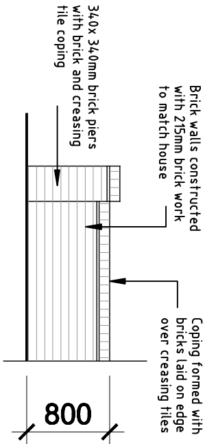
Brick Wall
