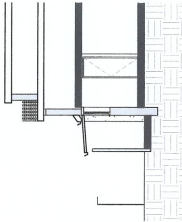
1 EXISTING SECTION A
