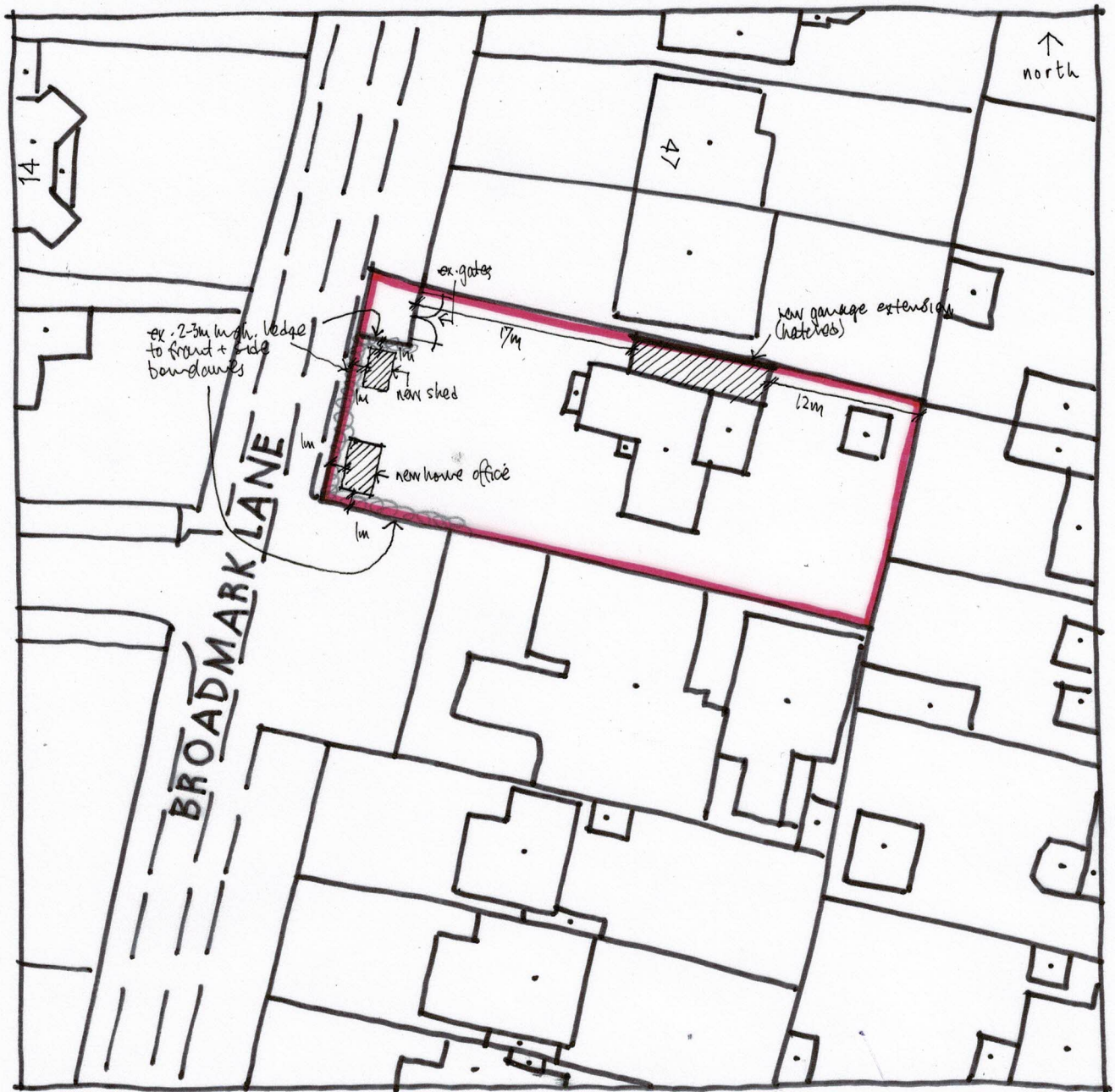
SITE PLAN 1:500 @ A4
