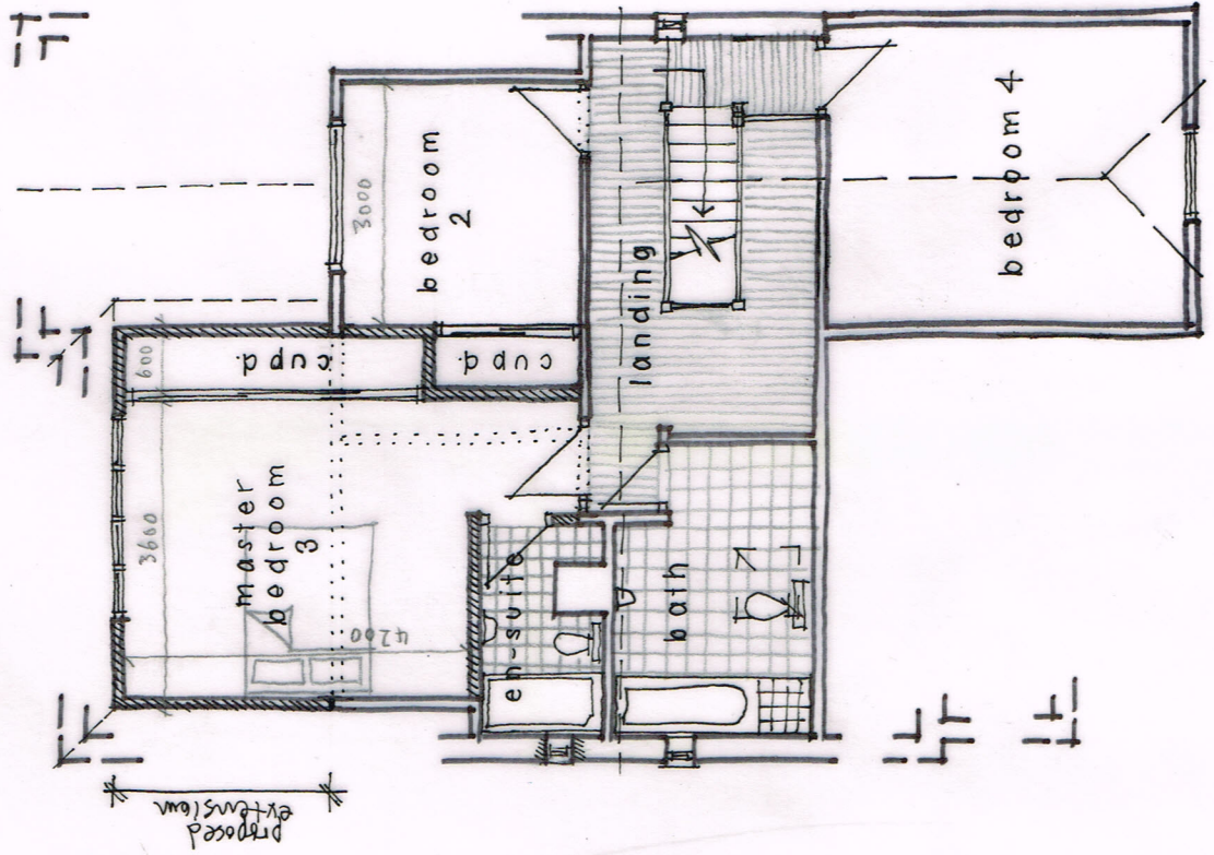
1st FLOOR PLAN 1:100 @ A3 / 1:50 @ A1
