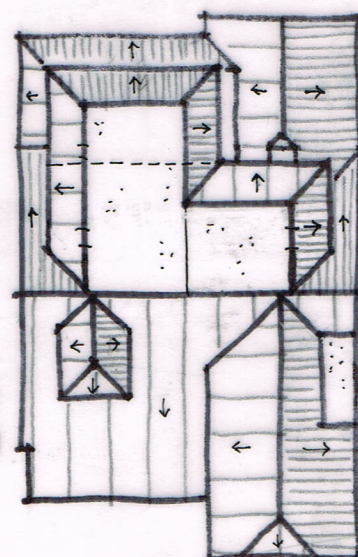
ROOF PLAN 1:200
