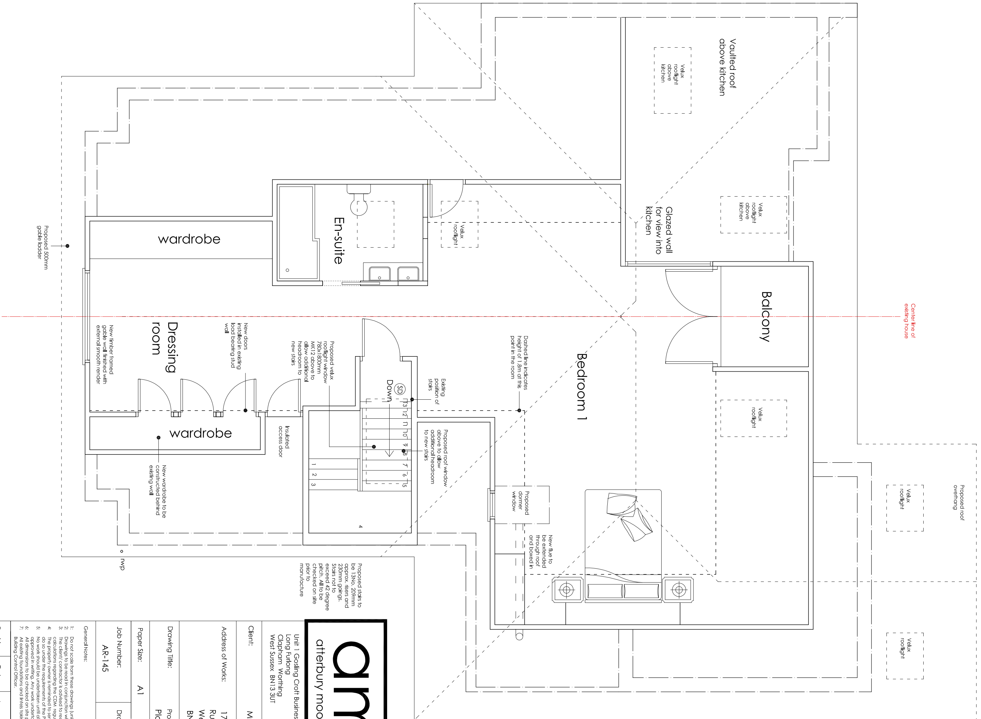
PROPOSED FIRST FLOOR PLAN 1:50
