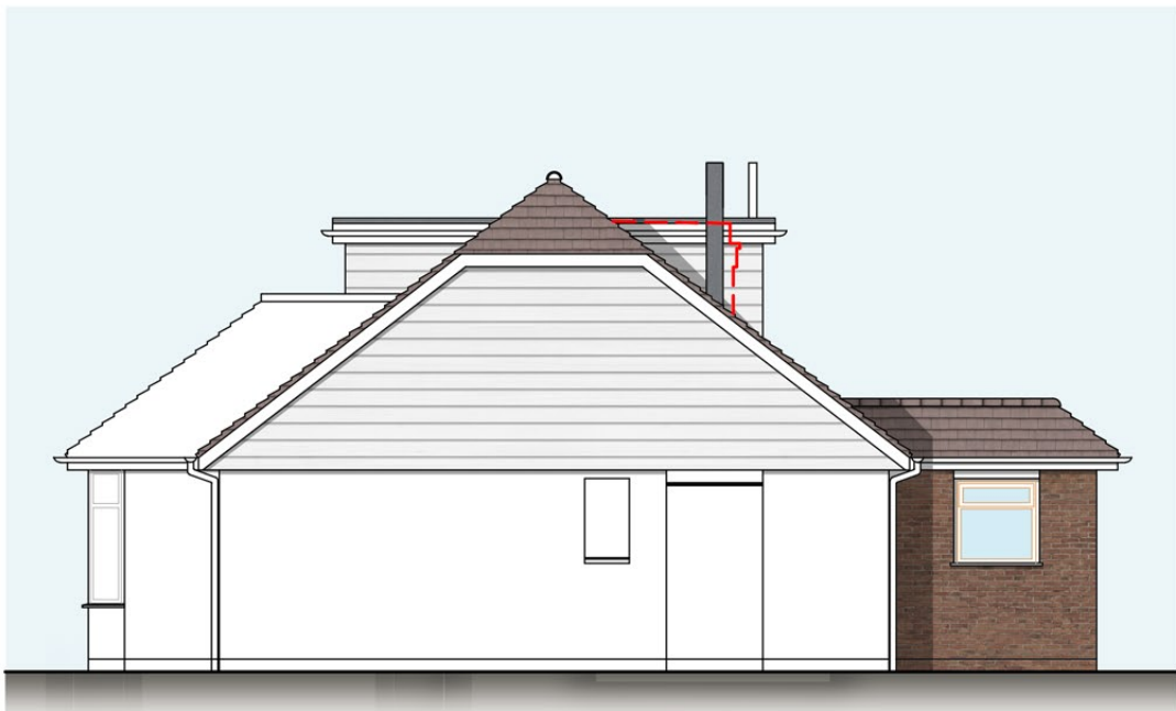
South Elevation – (Side) 1:100
