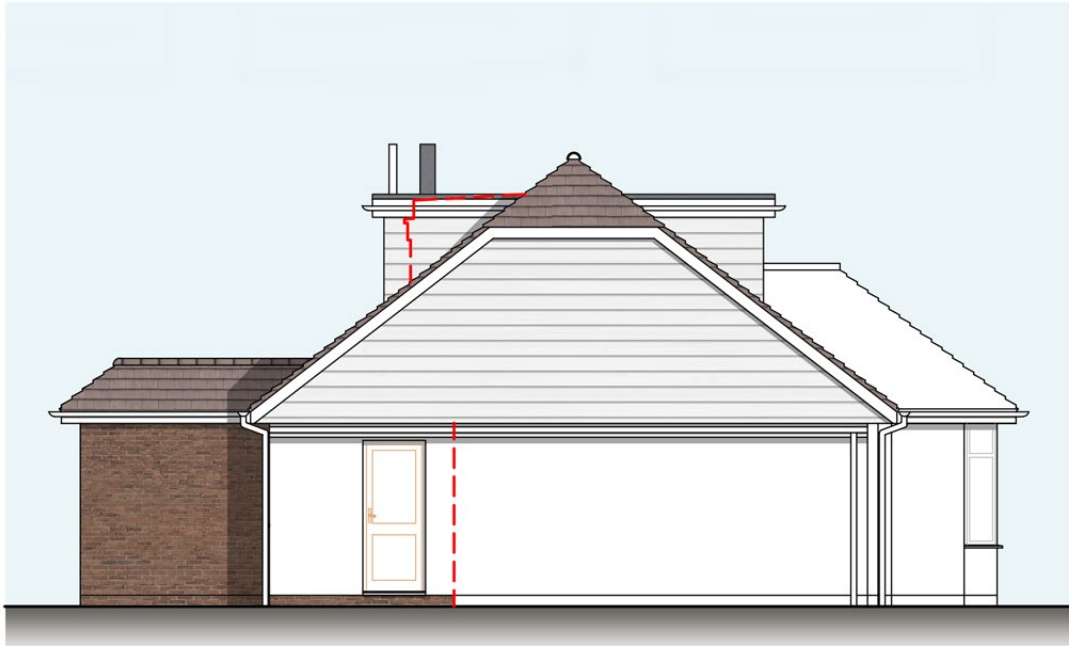
North Elevation – (Side) 1:100
