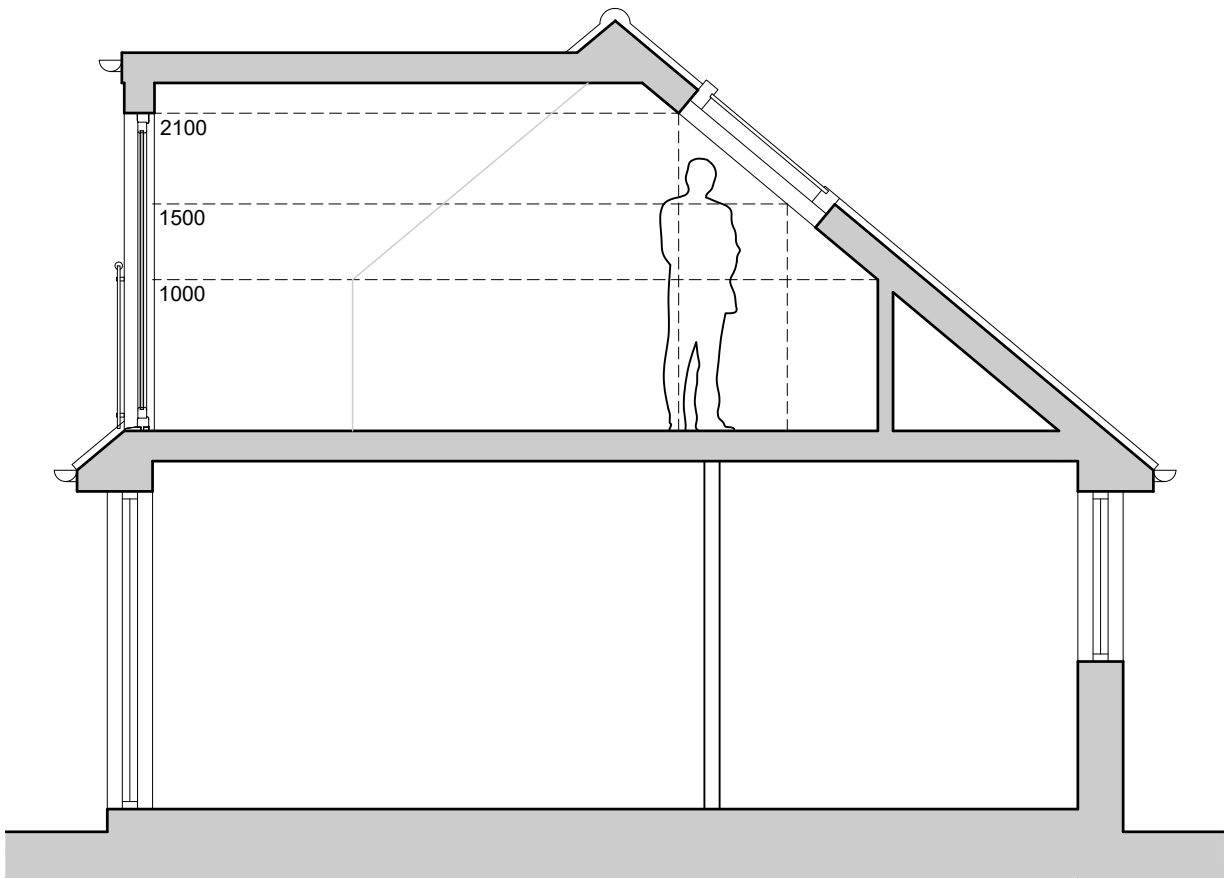
02 - Section
