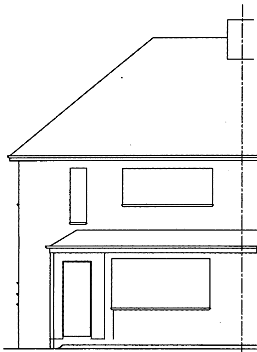
Front Elevation
