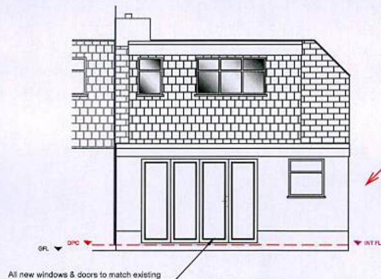
Rear Elevation
