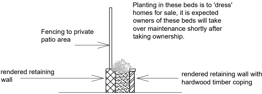
Section B-B 1:50
