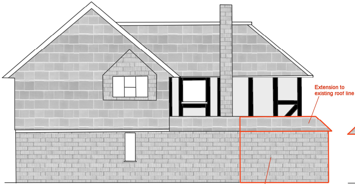
West Elevation
