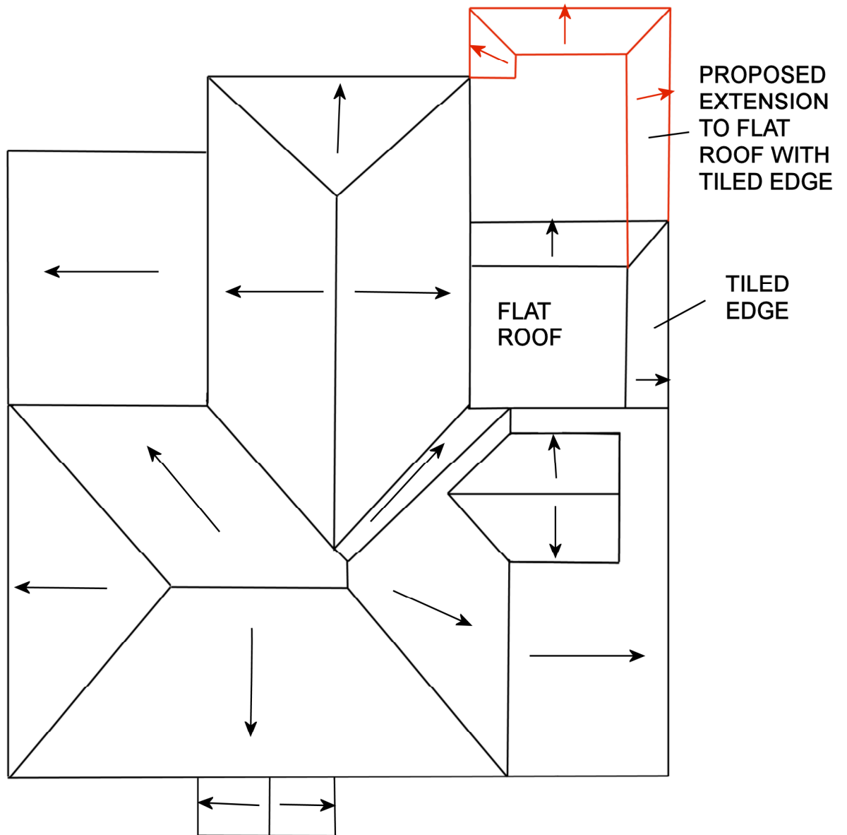
ROOF PLAN SCALE 1:100 at A4
