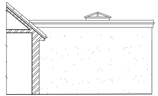
Side Elevation (South-East Facing) (Scale 1:100)
