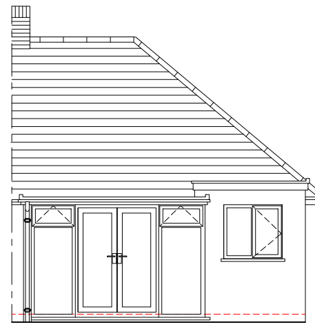
Rear Elevation (North-East Facing) (Scale 1:100)
