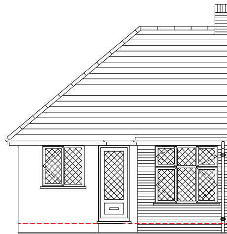
Front Elevation (South-West Facing) (Scale 1:100)
