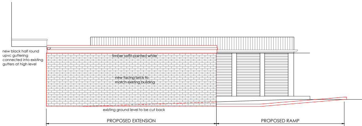
PROPOSED SOUTH FACING ELEVATION
