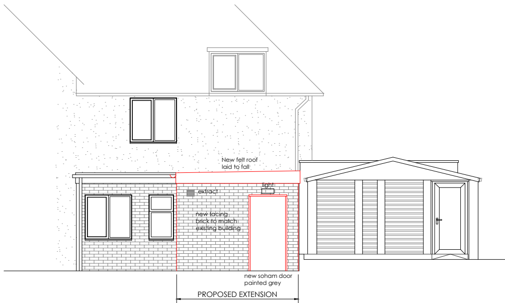
PROPOSED EAST FACING ELEVATION
