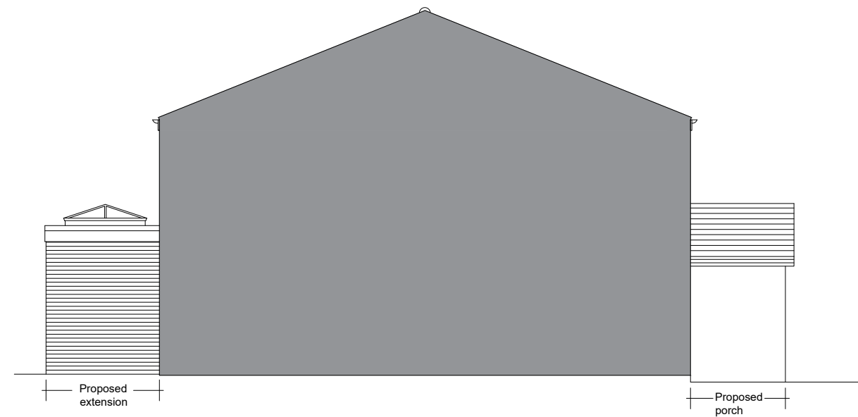
South Elevation
