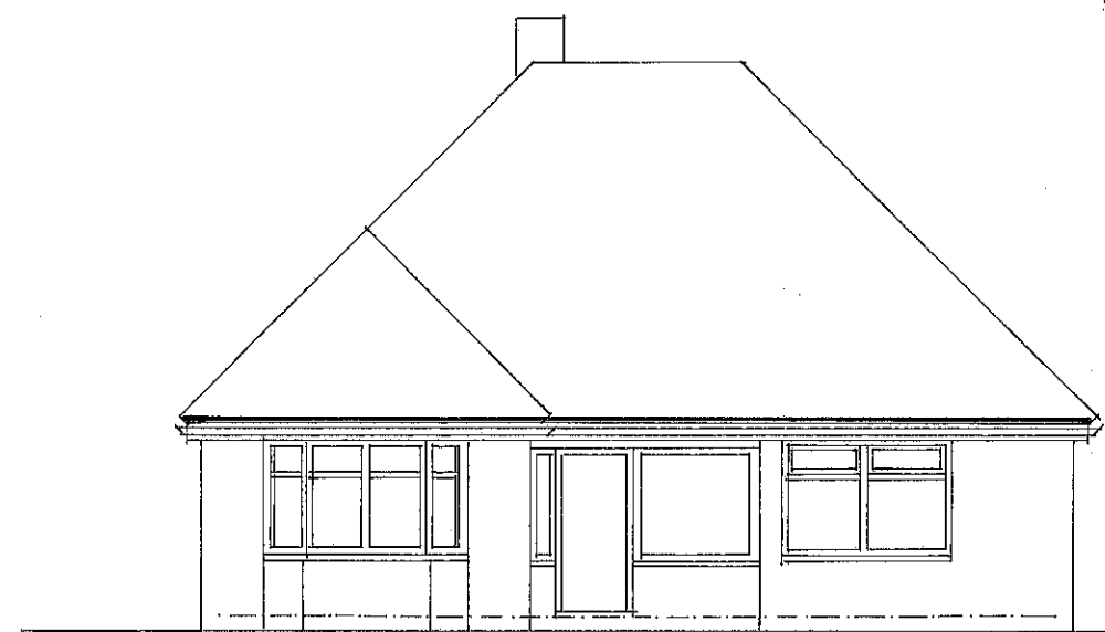
WEST ELEVATION TO DOLPHIN WAY
