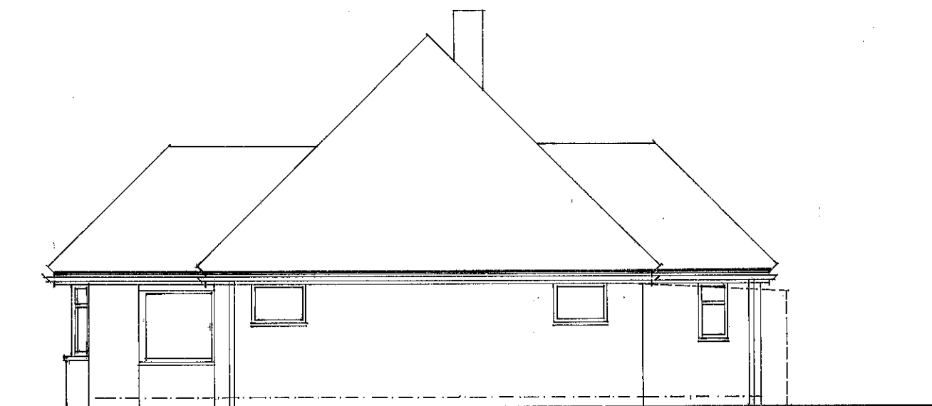
SOUTH ELEVATION
