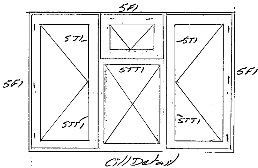
Office Window, Rear Elevation - Window No 6
