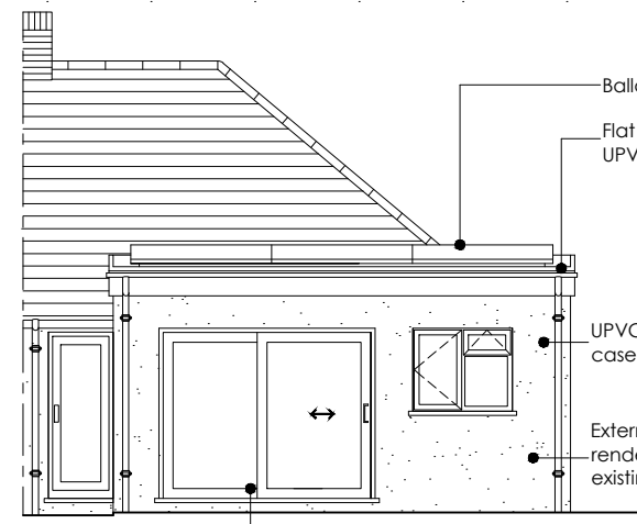
Rear Elevation (North-East Facing) (Scale 1:100)
