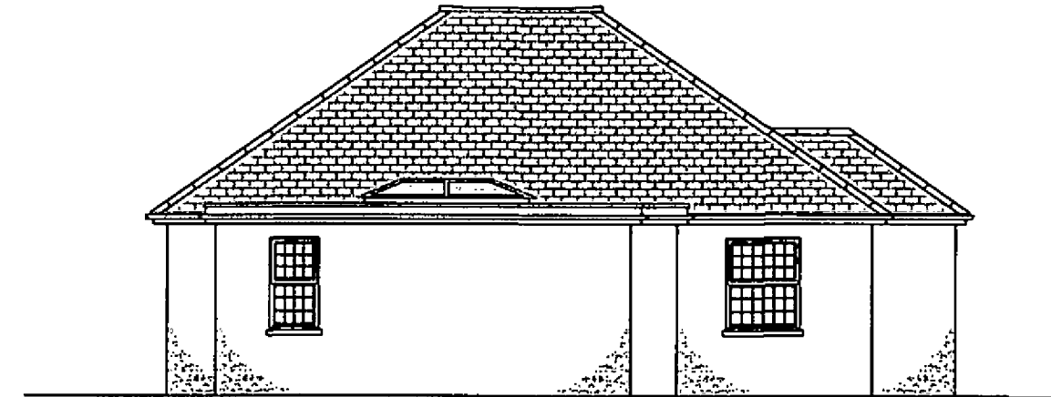
PROPOSED REAR ELEVATION (SOUTH)
