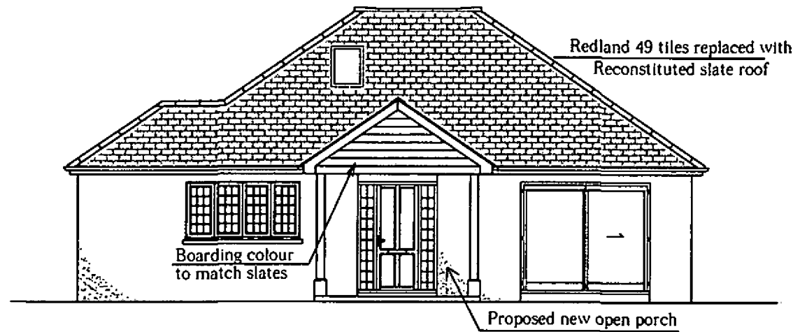
PROPOSED FRONT ELEVATION (NORTH)
