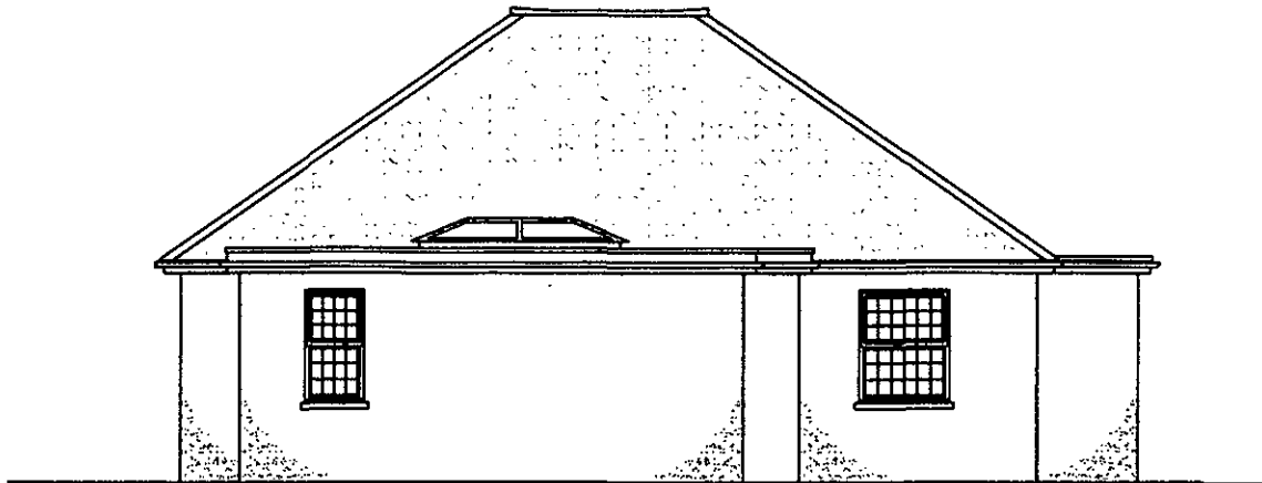
REAR ELEVATION (SOUTH)
