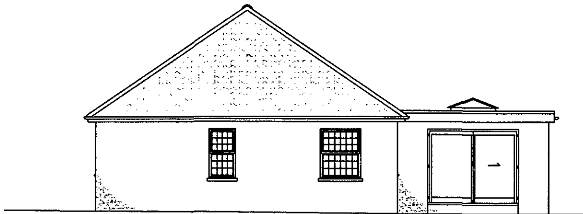
SIDE ELEVATION (EAST)
