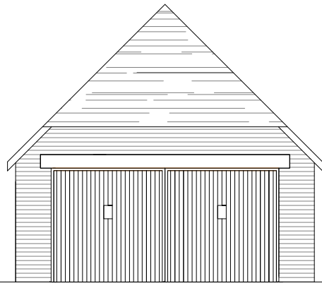
FRONT ELEVATION (WEST)
