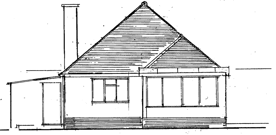
REAR ELEVATION (W)
