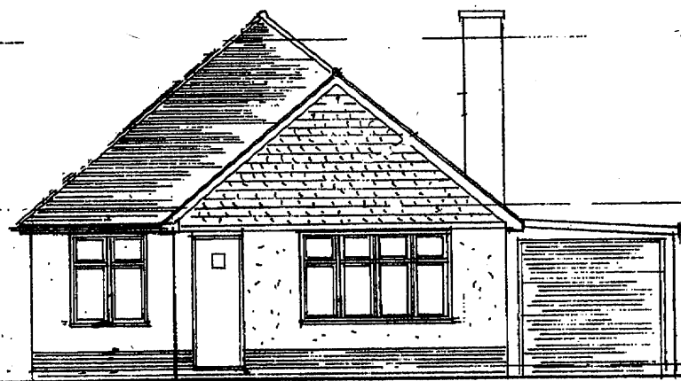
FRONT ELEVATION (S)
