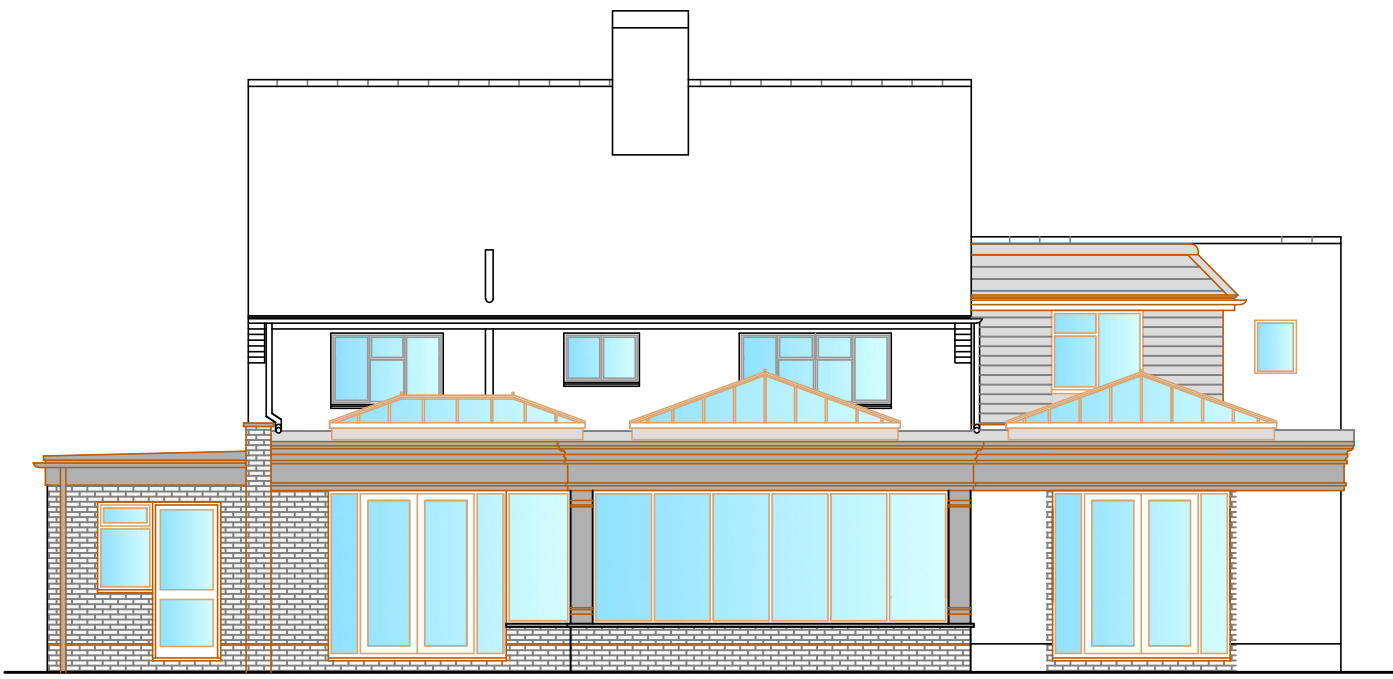
West Elevation (Rear)
