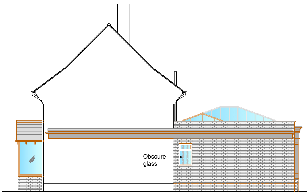
North Elevation (Side)
