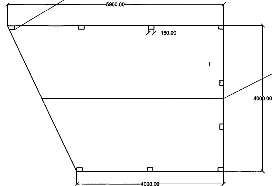
plan view
