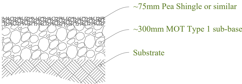
Typical Bund 1:50 | PROPOSED
