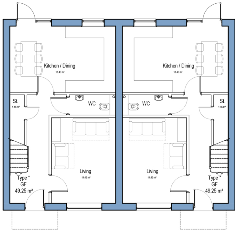
House Type G Ground Floor Plan 3 Bed / 5 Person House GIA: 98m²
