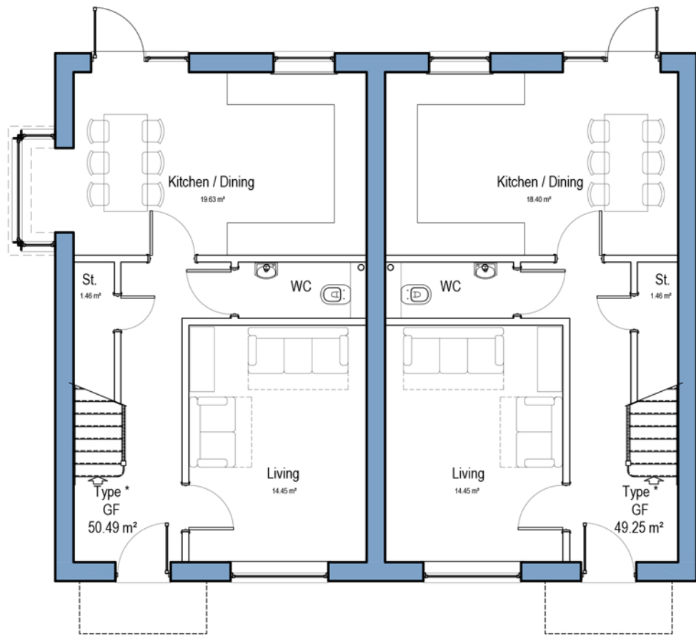
House Type G Ground Floor Plan 3 Bed / 5 Person House GIA: 98m²
