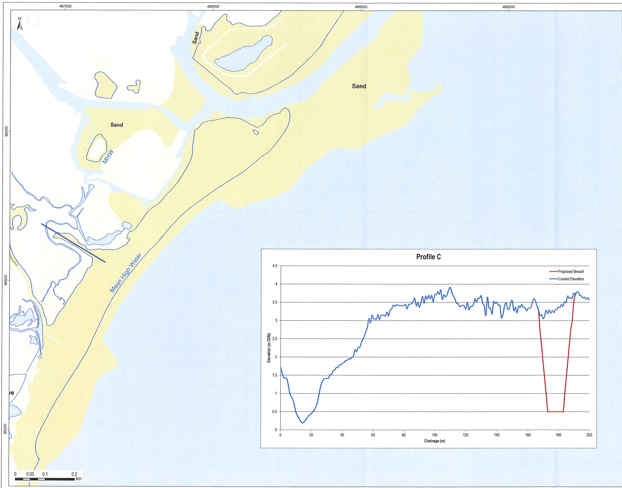
Cross-section Plan of the Tern Island Breach
