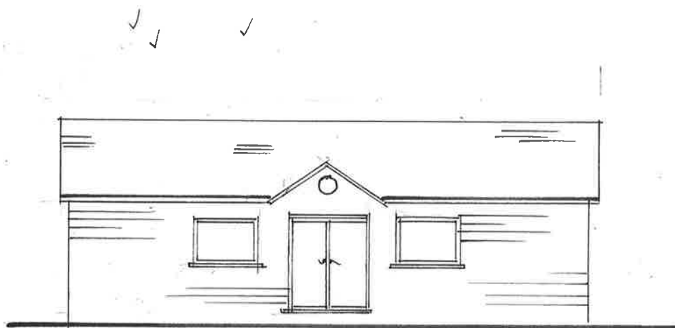
SOUTH ELEVATION
