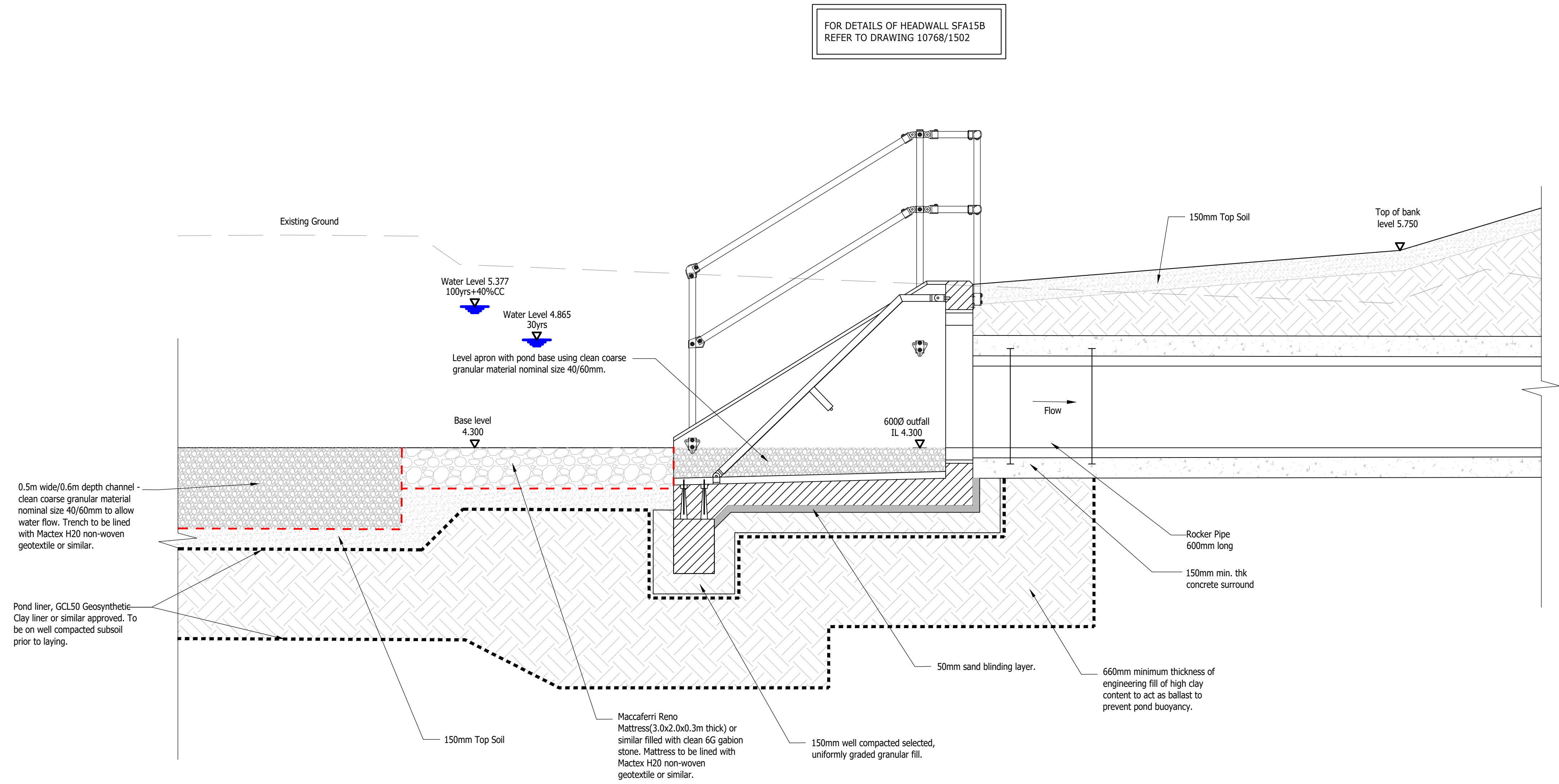
Detention Basin 5 Section J-J Scale 1:20
