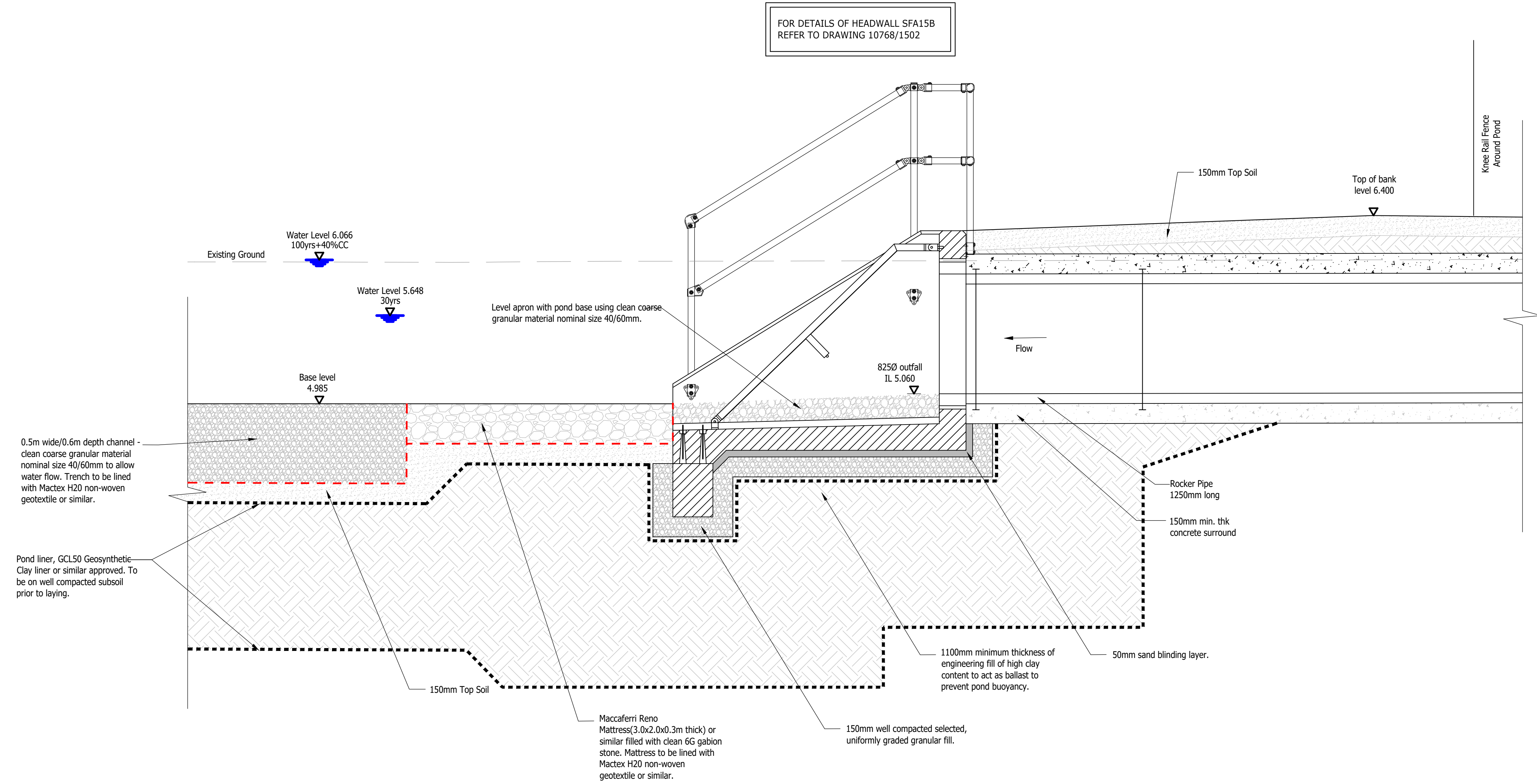
Detention Basin 1 Section A-A Scale 1:20
