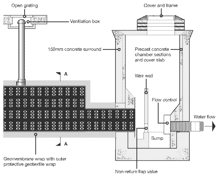
Typical vent detail
