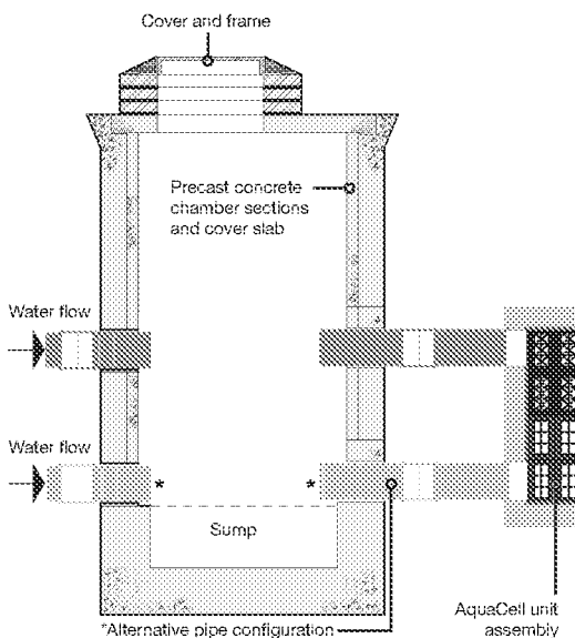
Long section
