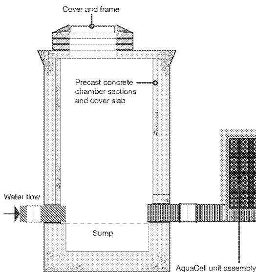
Long section
