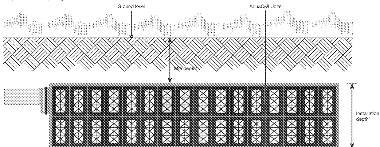
Trench soakaway
