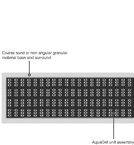
Long section
