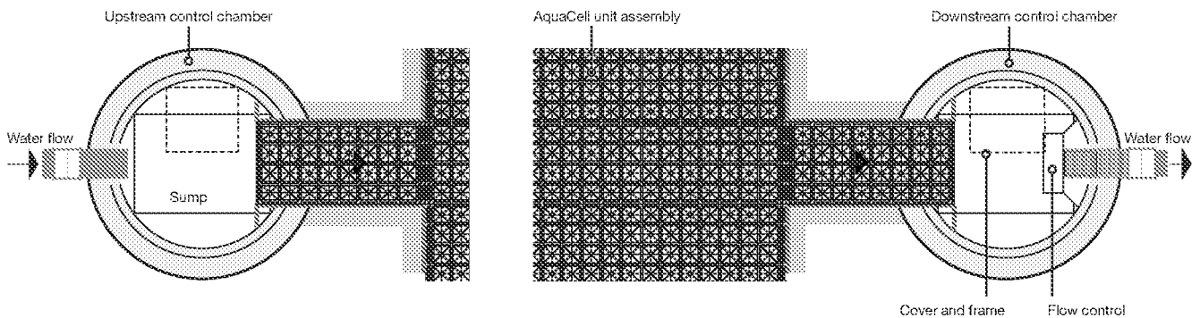
Plan
