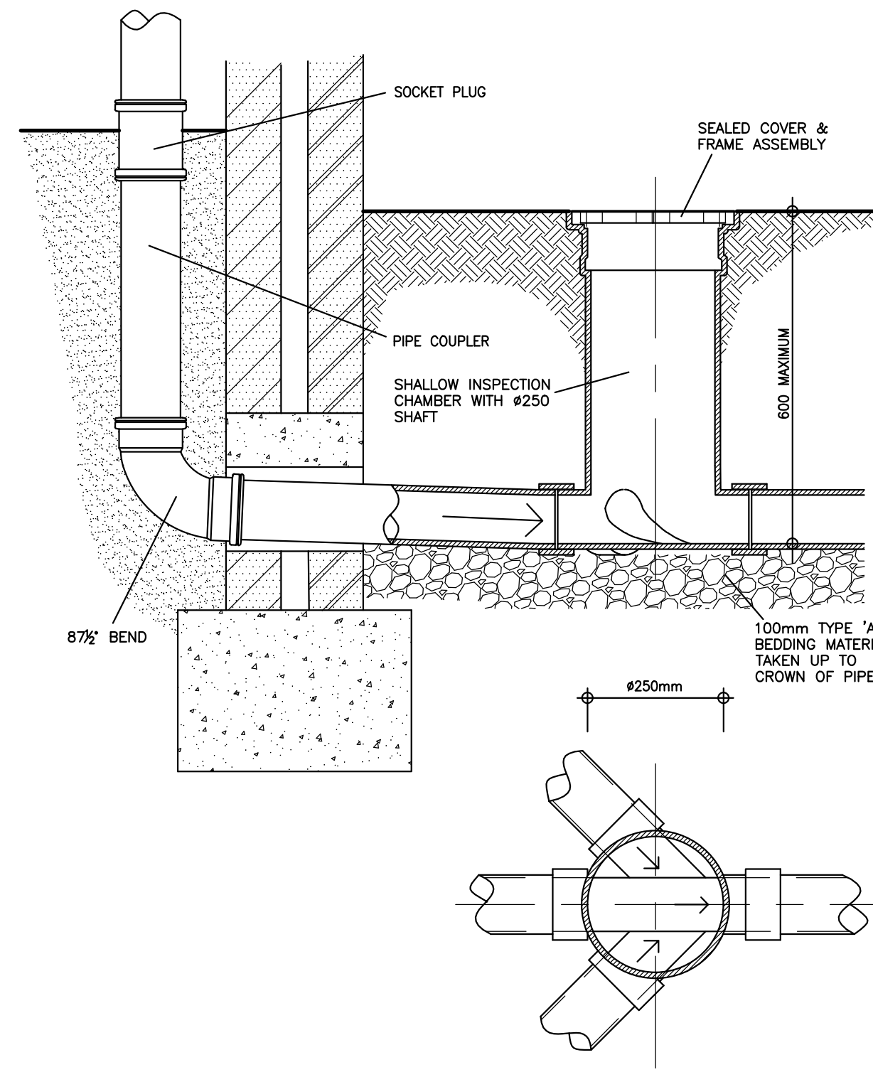
TYPICAL SHALLOW ACCESS INSPECTION CHAMBER (1:10 typical)
