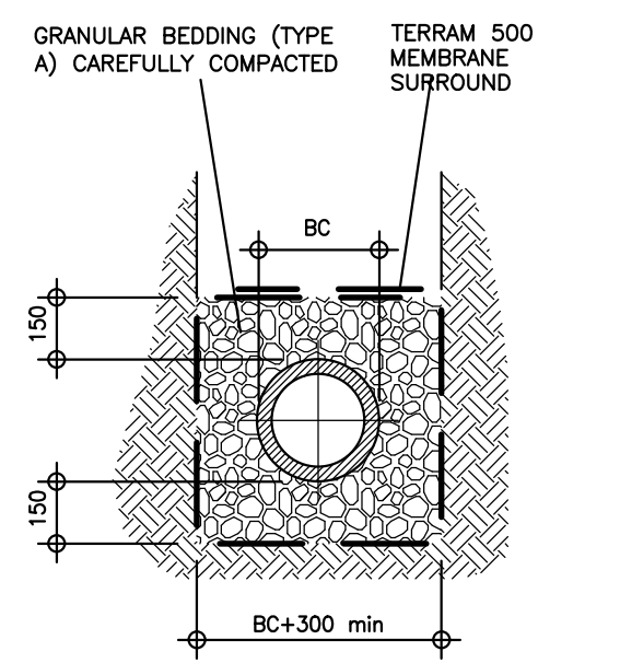
GRANULAR SURROUND TO BE USED WHERE PIPE PASSES WITHIN 3M OF NEW OR EXISTING TREES UNLESS PIPE REQUIRED CONCRETE SURROUND
