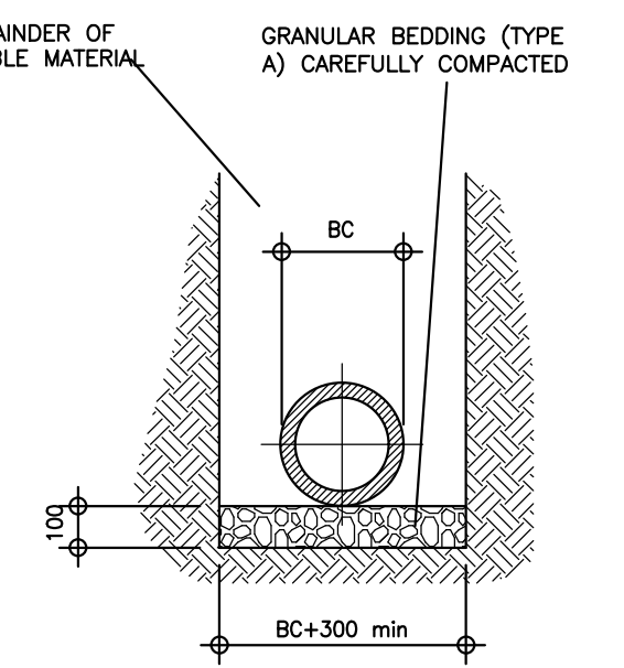
GRANULAR BED TO BE USED WHERE COVER TO CROWN OF PIPE IS GREATER THAN 600mm IN LANDSCAPED AREAS
