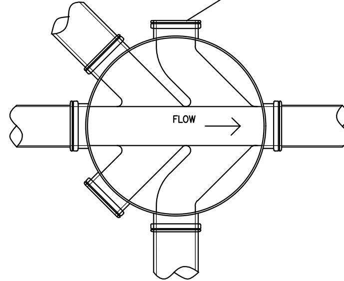
TYPICAL INSPECTION CHAMBER (1:10 typical)
