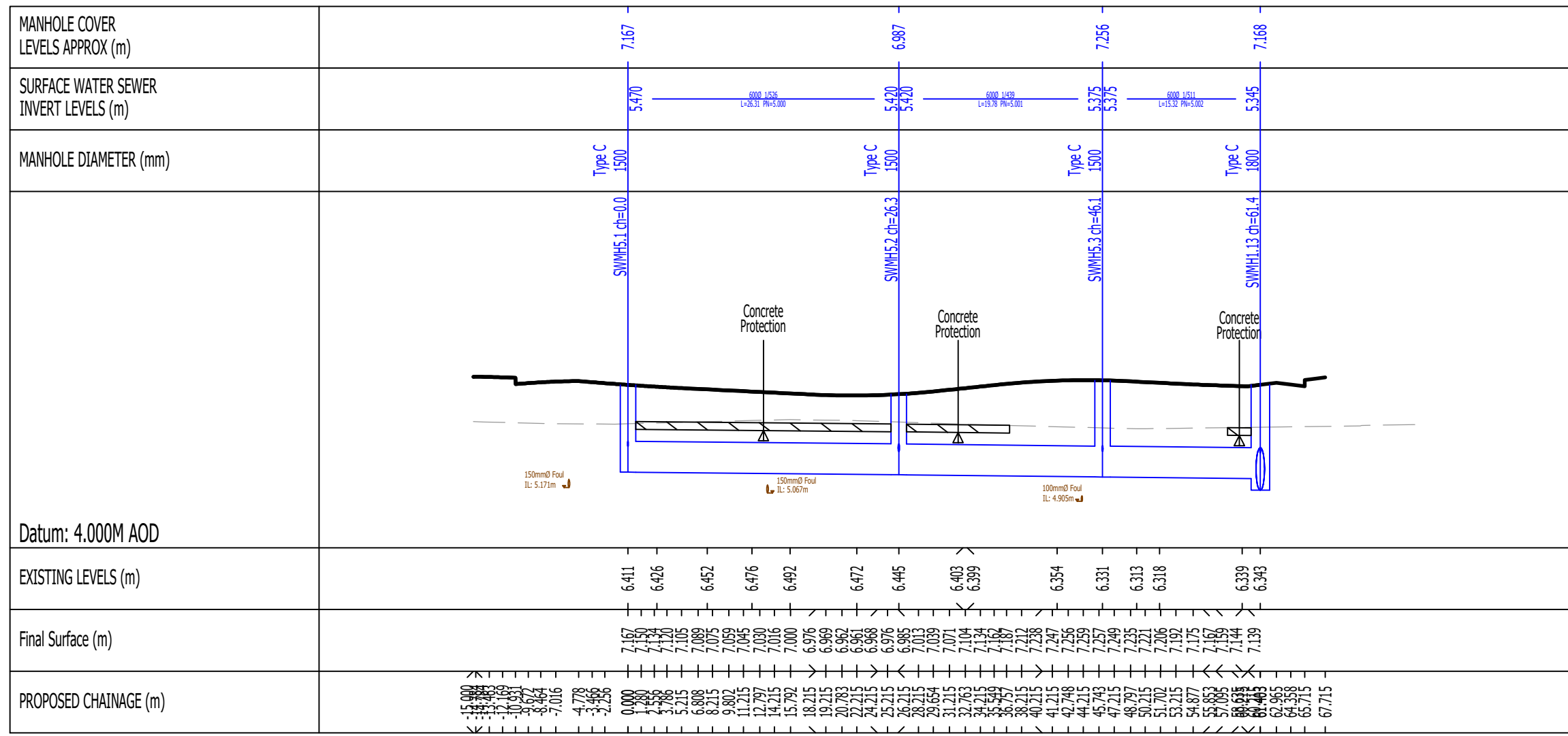
SWMH5.1 - SWMH1.13 LONG SECTION
