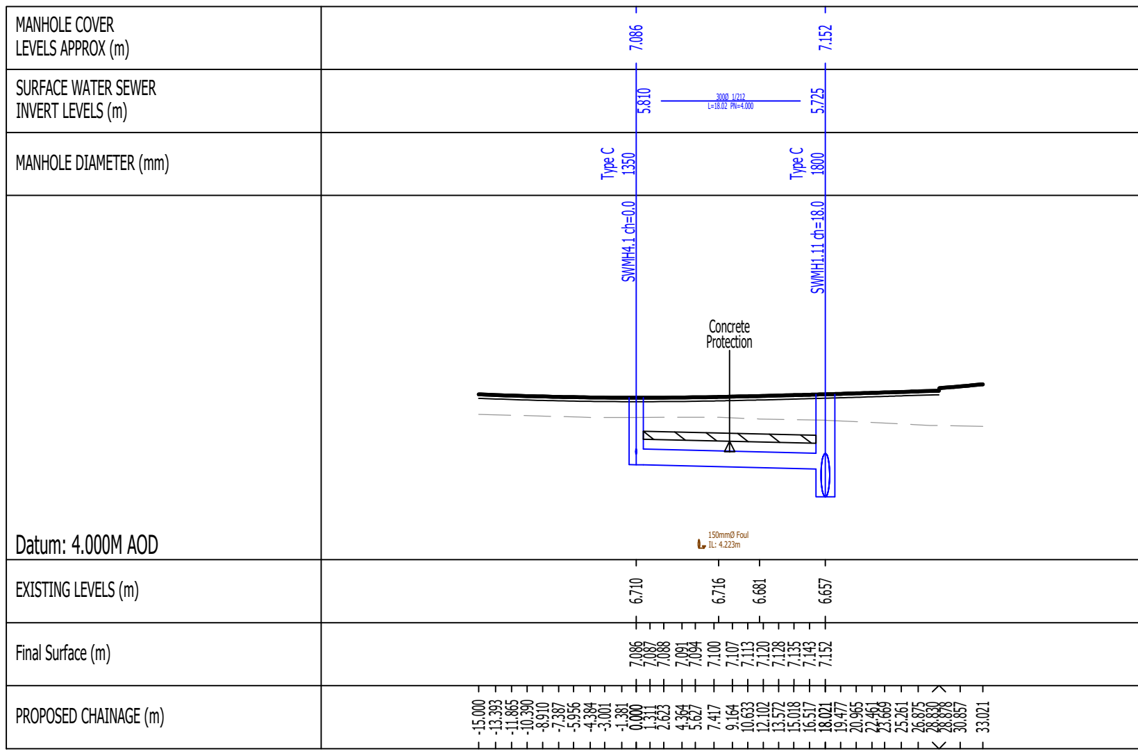
SWMH4.1 - SWMH1.11 LONG SECTION
