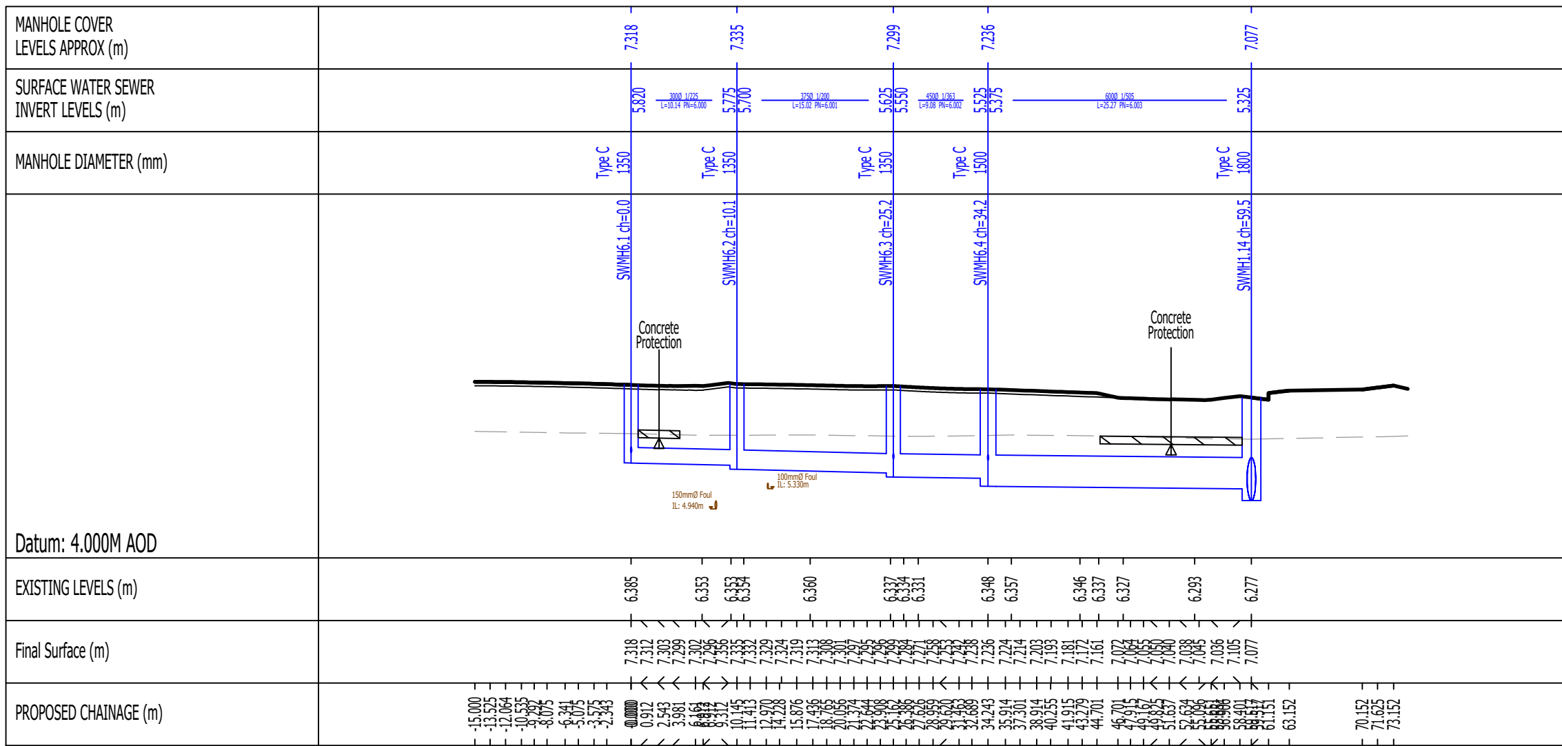
SWMH6.1 - SWMH1.14 LONG SECTION
