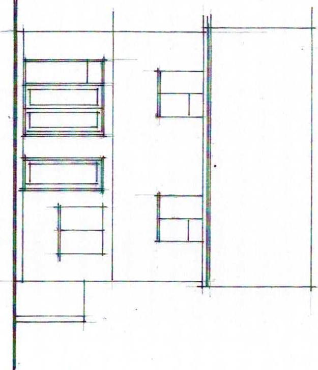
EAST ELEVATION 1-100
