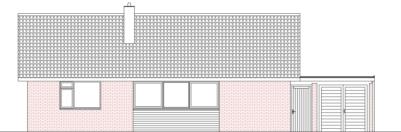
FRONT ELEVATION
