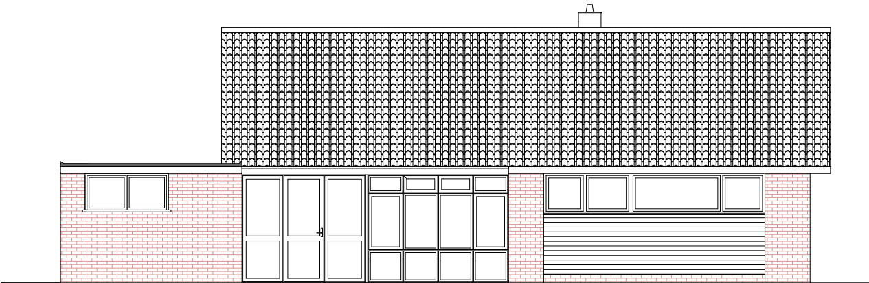
REAR ELEVATION
